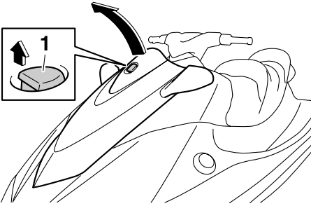
1 Hood latch
